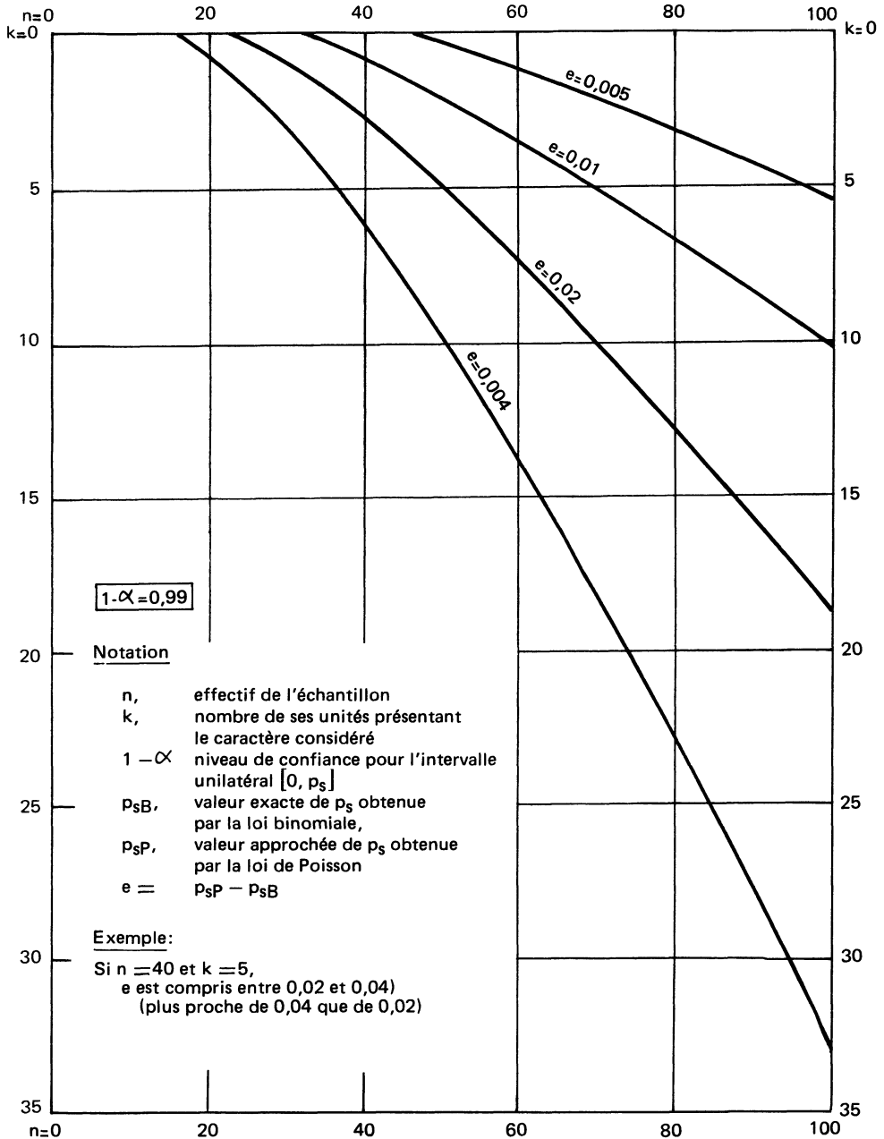
Abaque 4
