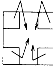
FIG. 9.3 - \dim_H \Lambda(\Gamma) = \log 4 / \log(1/\alpha) .
