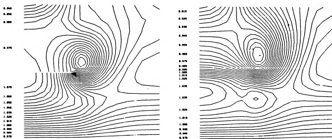
Figure 9. Isobars in cross-planes at 60% of the plate and at the trailing edge for M_\infty = 0.7 and \alpha = 30^\circ
