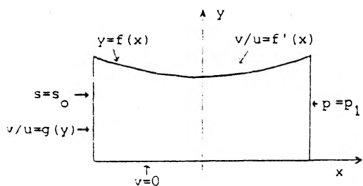
Fig.11. Boundary conditions.
