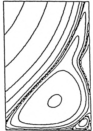
Appearance and disappearance of small eddies for Re = 11000 with the 256 x 256 grid
