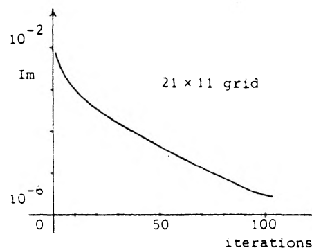
Fig.12. Convergence history ( p_1 = 1.08 ).
