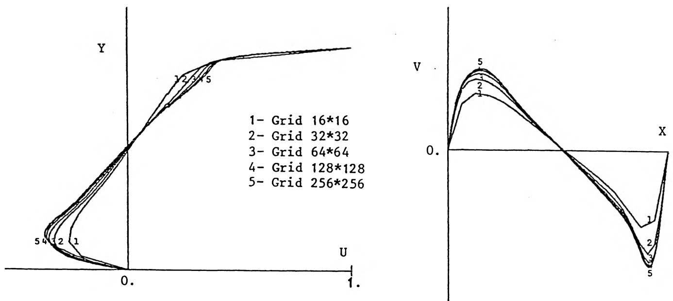
Re = 1 000 Evolution of velocity profiles along centerlines with different grids FIGURE 4
