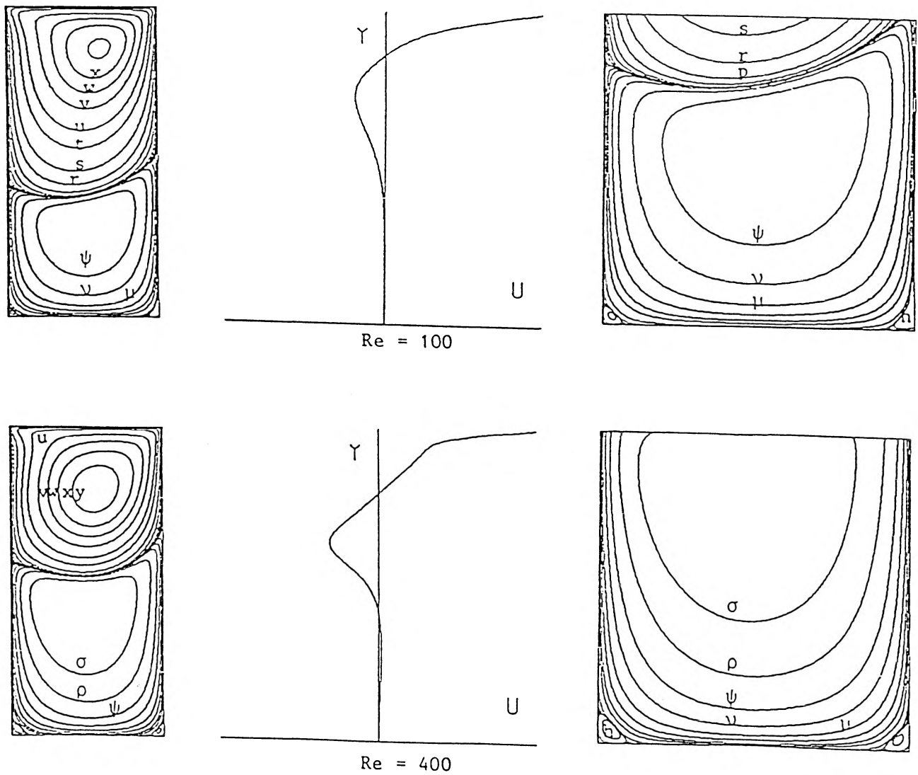
Streamlines and u velocity profile along centerline in the rectangular cavity
