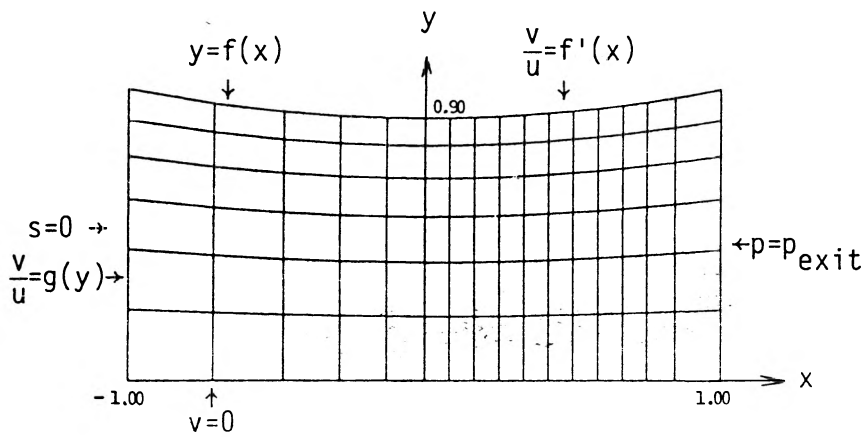
Boundary conditions and mesh for the nozzle
