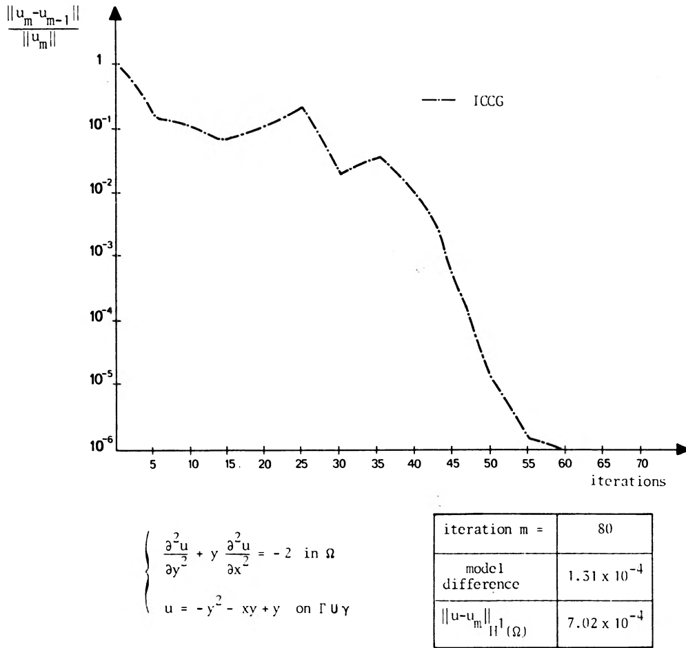
Fig. 9. Solution of Tricomi's problem with the 7(b) grid.
