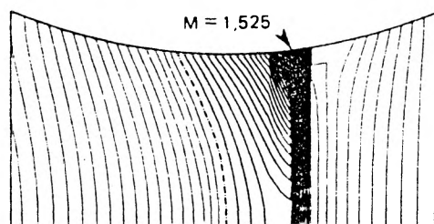
Fig.10. Iso-Mach lines for an exit density = 1.35 ( \Delta M = 0.025 ) -- sonic line
