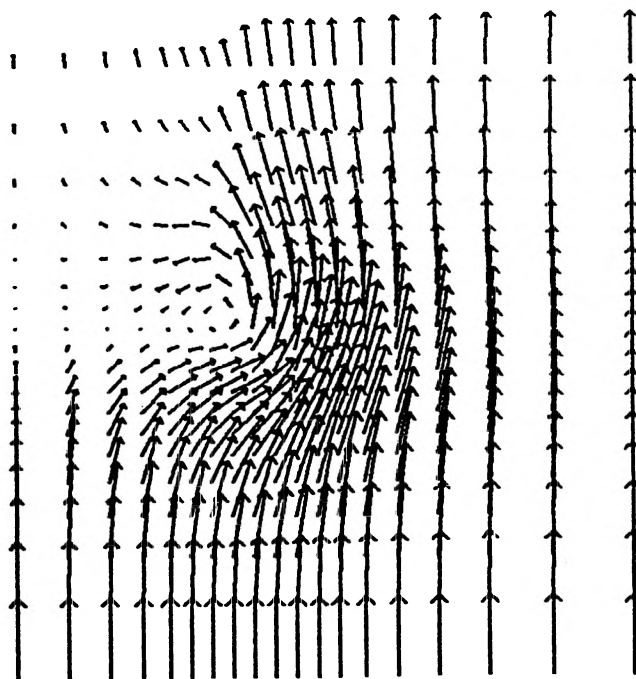
Figure 10 Cross-flow velocities at 110 % of the plate.
