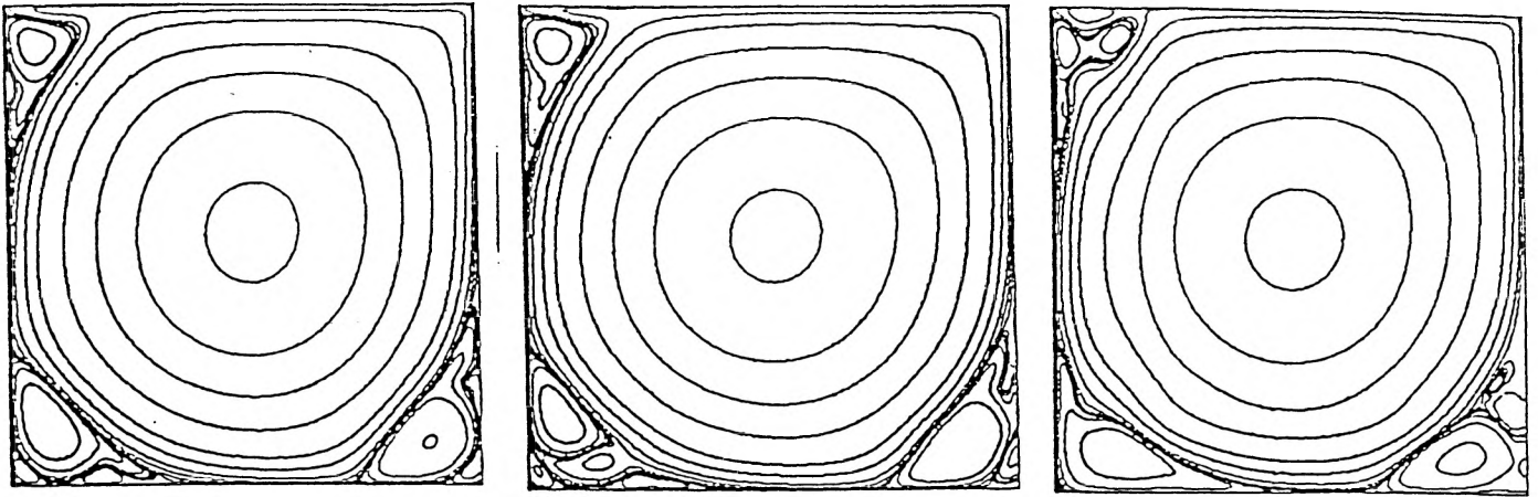
Evolution of the solution during iterations for Re = 10000 with the 512x512 grid
