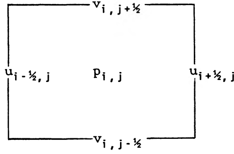
Pressure and velocity in the cell (i,j) Figure 1
