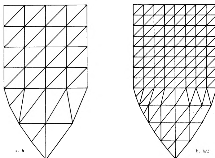
Fig. 7. Grids for Tricomi's problem.
