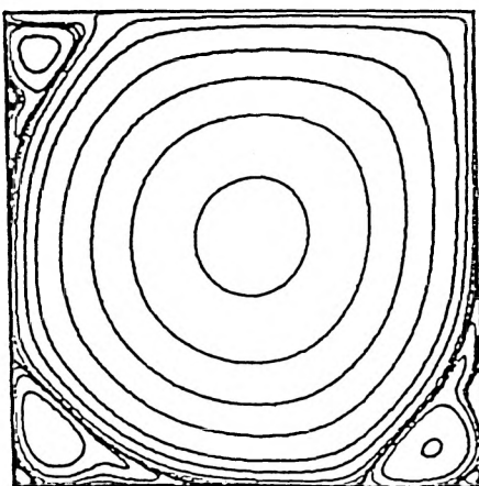
Appearance and disappearance of small eddies for Re = 11000 with the 256 x 256 grid
