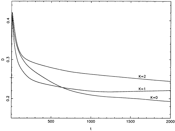
Fig. 7. – Time-dependence of the diffusion coefficient of the process y_t - y_0 , computed along three different orbits. The quantity K , is defined as K = (y_T - y_0)/N represents the number of times the orbit has wrapped around the torus in the y -direction.
