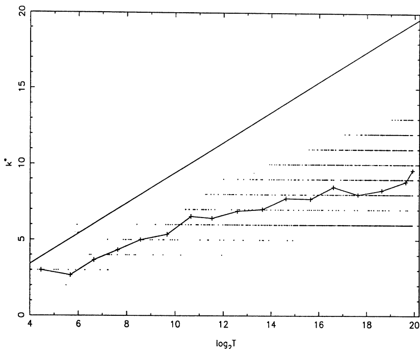
Fig. 8. – Breaktime for exponential growth of the complexity of the sequence \epsilon(x_t) , for the golden mean rotation number, and various orbits (scattered points). The broken line represents an average. The solid line is the breaktime for a pseudo-random sequence of the same length of the doubling map, for comparison.
