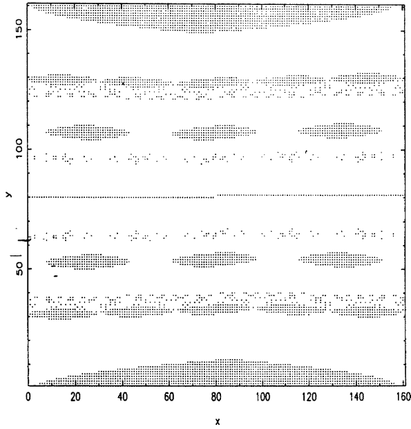
Fig. 1. – Phase portrait of the mapping (1) for \lambda = 1/N , and N = 161 , showing several orbits. Some low-order rotation numbers support stable resonant regions (i.e., 0, 1/3 , 1/5 ), while others do not (i.e., 2/5 , 1/4 ). The invariant set at the rotation number 1/2 , is a quasi-torus.
