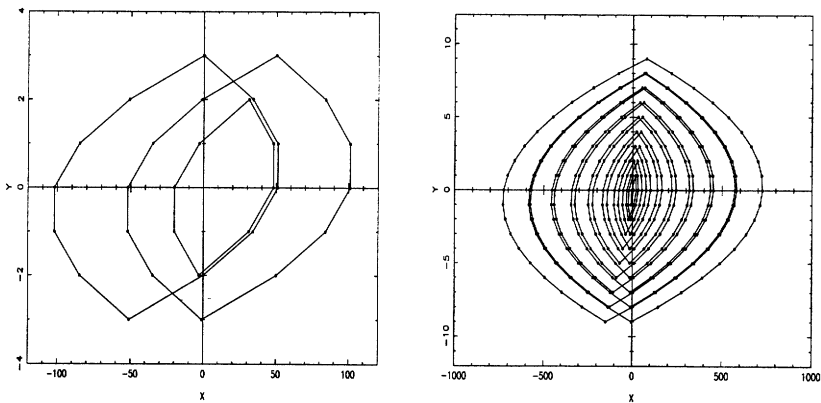
Fig. 2. – Elliptic-type orbits of the local mapping (7) for n = 17 . Left : three orbits of unit index, corresponding to \sigma = 0 . Note the discontinuous nature of the half-period function F_+ , defined in (19). Right : a single orbit of index 17, for \sigma = 4 .
