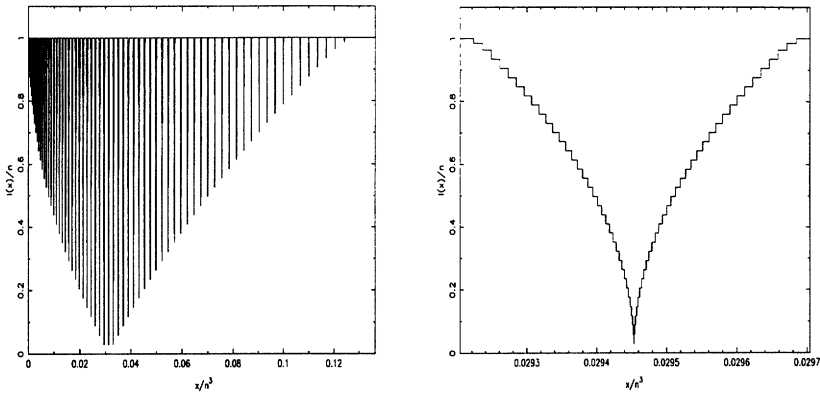
Fig. 4. – Left : The index function I(x) vs. the amplitude x , for a resonance of prime order n = 137 . Both coordinates are normalized. The value of the shift \sigma = (n+1)/4 corresponds to the primary peak of the critical amplitude (cf. Figure 3, left). Right : enlargement of one of the three deepest canyons, showing its detailed structure. The bottom of the canyon corresponds to a point of index 4 (the middle canyon contains two points).
