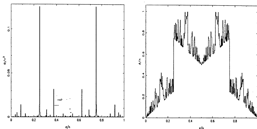
Fig. 3. – Critical amplitudes vs. shift for the resonances of prime order n = 419 . All quantities are normalized. Left : Maximal amplitude. Right : Minimal amplitude.
