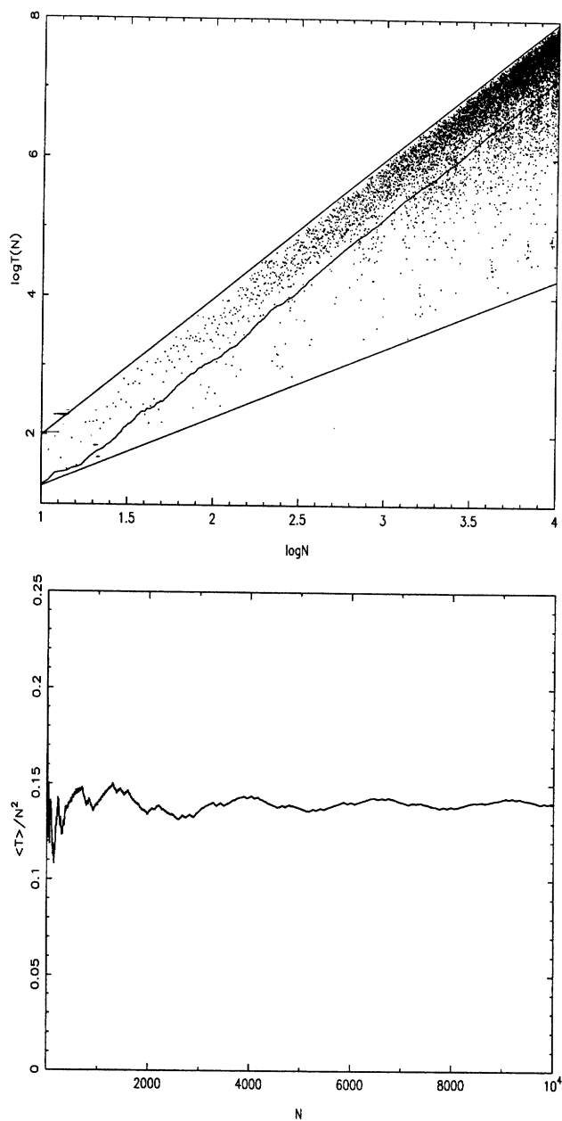
Fig. 6. – Maximal period of the orbits, on a lattice of size N , for the golden mean rotation number. Top : the period function T(N) , with upper and lower envelopes, and its average order \langle T \rangle . Bottom : normalized average order \langle T(N) \rangle / N^2 .
