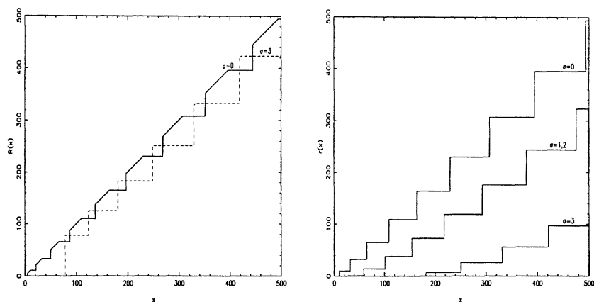
Fig. 5. – Dependence of the radii of maximal invariant set on the amplitude, for some resonances of prime order n = 11 . Left: Outer radius R(X) for \sigma = 0 and 3. Right: Inner radius r(X) , for \sigma = 0, \dots, 3 .
