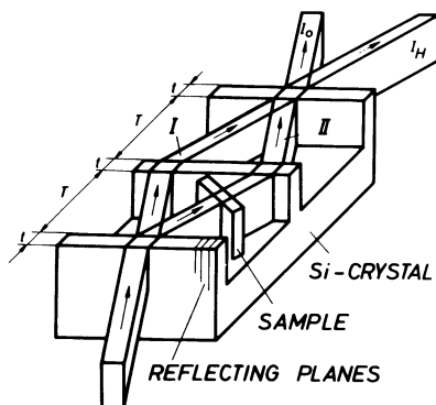
FIG. 1. — Sketch of the standard symmetric perfect crystal interferometer.
