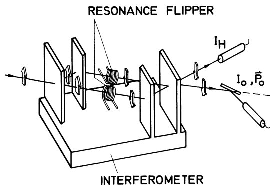
FIG. 3. — Sketch of the double resonance coil experiment.
