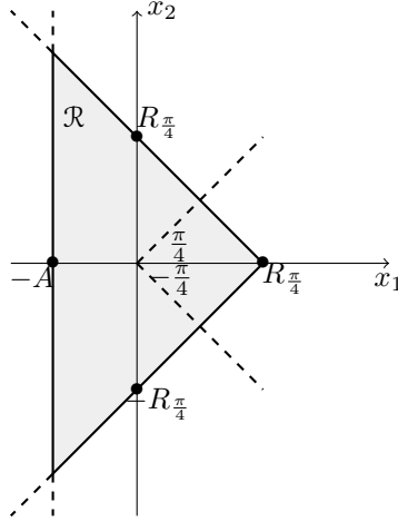
FIGURE 2. \mathcal{R} is a compact set of \mathbb{R}^2 .
