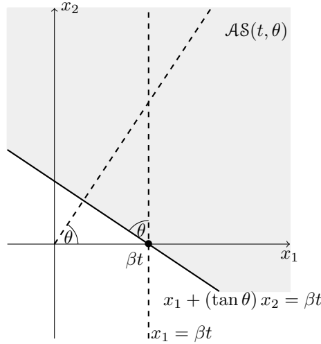
FIGURE 1. \mathcal{AS}(t, \theta) := \left\{ (x_1, x_2) \in \mathbb{R}^2 : x_1 - \beta t + (\tan \theta) x_2 > 0 \right\} .
