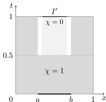
FIGURE 1.1. The function \chi decreases to zero in I'
