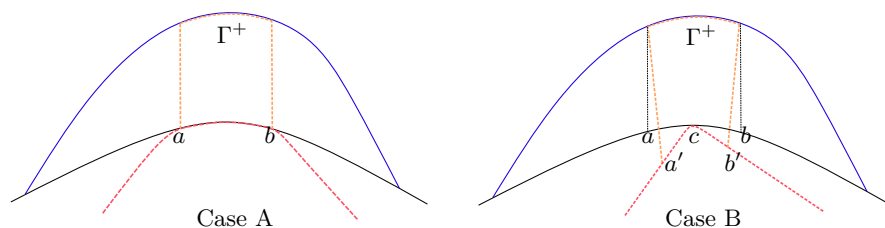
FIGURE 4. Case A. \partial_i^D \Omega \cap \partial E(\hat{\sigma}) = \widehat{ab} . The dotted curve upon \Omega represents \Gamma^+ in (5.17). Case B. \partial_i^D \Omega \cap \partial E(\hat{\sigma}) = \{c\} . The dotted curve upon \Omega represents the curve \Gamma^+ in (5.20).
