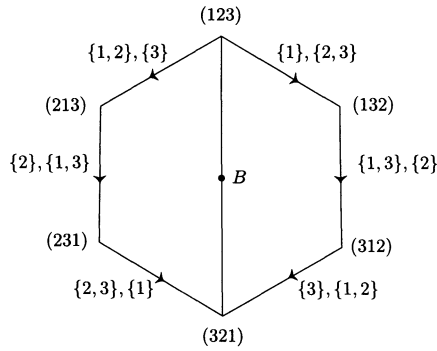
Figure 1. The geodesic and barycenter of P_3
