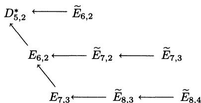
Diagram 3. Classification tree 3
