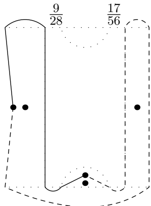
Image under \xi'_{6,9/28}
