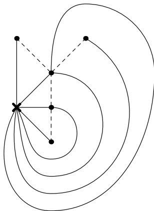
An example of a graph
