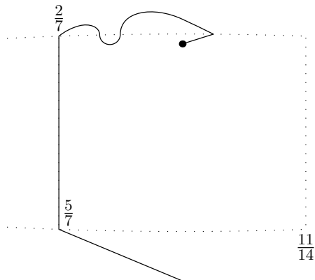
The path \beta'(w'_5) , after modification.
