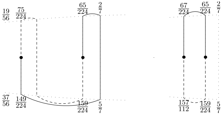
U(\beta(w_6), \beta(w_7)) and U(\beta(w_7), \beta(w_3)) .
