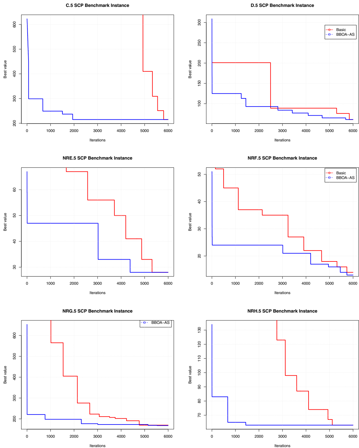
FIGURE 6. Convergence charts for the most difficult instances of the test groups: C, D, NRE, NRF, NRG, and NRH.
