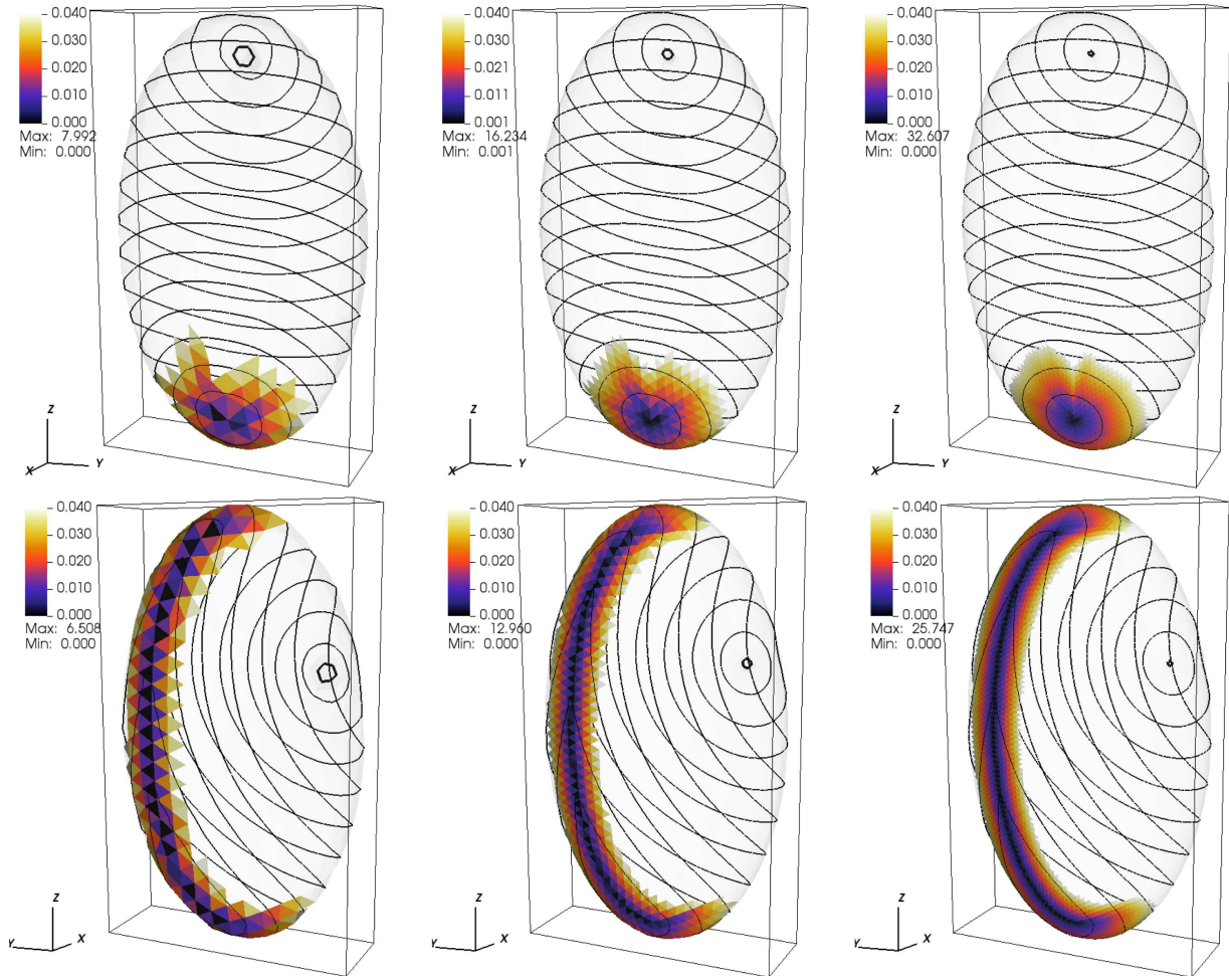
FIGURE 4. Ellipsoid (x/0.2)^2 + (y/0.6)^2 + (z)^2 = 1 . Upper panels: spatial distribution of \mu_h^* for the point p^1 = (-0.115470, 0, 0.816497) . We report the results for three meshes, one the conformal refinement of the other, with the first having 534 nodes and 1064 triangles, and the latter 8514 nodes 17024 triangles. The point p^1 is located “behind” the visible ellipsoid and it is marked with a black circle. We report only those triangles where \mu_h^* is below 0.04. We also report the contour lines of u_h^* . Lower panels: same plots for the point p^2 = (-0.151128, -0.350718, 0.295520) .
