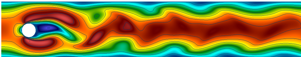
FIGURE 25. First component of the velocity solution to the Navier–Stokes problem on \Omega , obtained at the 484th iteration of the Schwarz algorithm, at T = 6 s, in the case of 4 subdomains.
