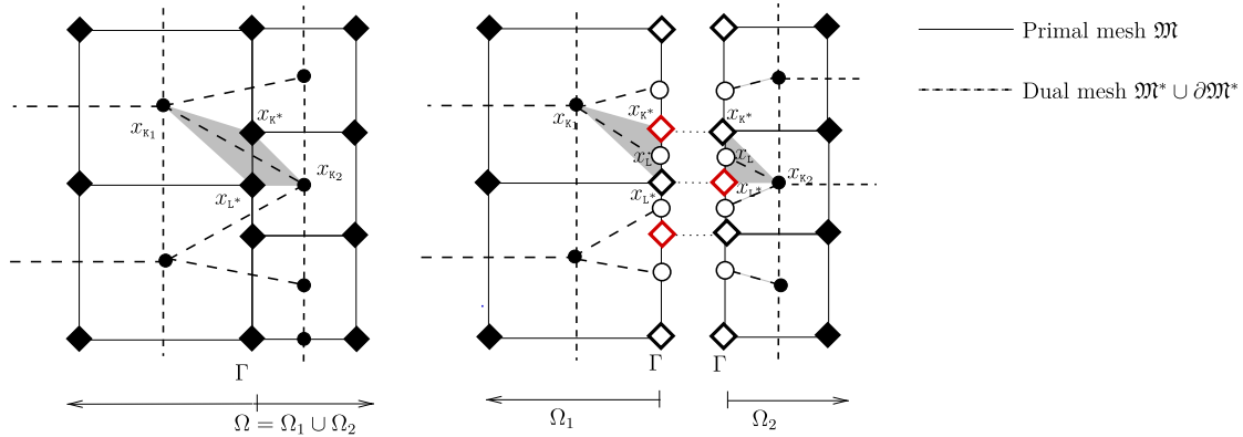
FIGURE 4. DDFV meshes.
