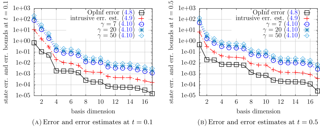
FIGURE 8. Convection-diffusion equation (Sect. 4.3.2). Increasing \gamma leads to a more conservative learned error estimate (3.18) for fixed M, J with respect to the intrusive error estimate. This simultaneously corresponds to a larger lower bound probability P^{\text{LB}} . The parameters used were M = 10 and \gamma = 7, 20, 50 for which P^{\text{LB}} \approx 0.75, 0.9985, 0.9999 .
