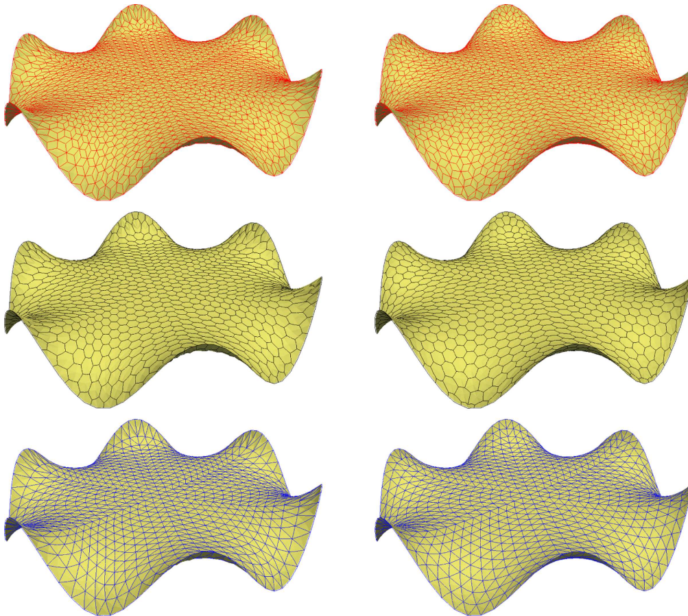
FIGURE 37. The evolved surface with sinusoidal boundary in time step n = 400 . Left column: the case with no tangential redistribution. Right column: the case with asymptotically uniform redistribution with \omega = 100 . First row: the diamond mesh, second row: the mesh of F -covolumes and third row: depicts the mesh of T -covolumes.
