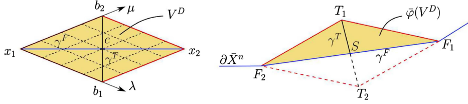
FIGURE 13. Left panel: the local coordinates on an inner diamond cell on X . Right panel: a boundary diamond cell on \tilde{X}^n .
