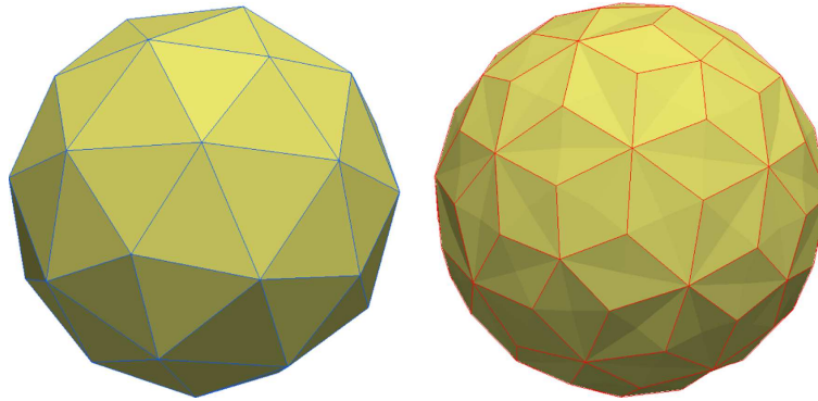
FIGURE 12. The discretization of the sphere S^2 embedded in \mathbb{R}^3 . Left panel: the triangular mesh \bar{X}^n for the cotangent scheme. Right panel: the diamond mesh \bar{X}^n for the DDFV method.
