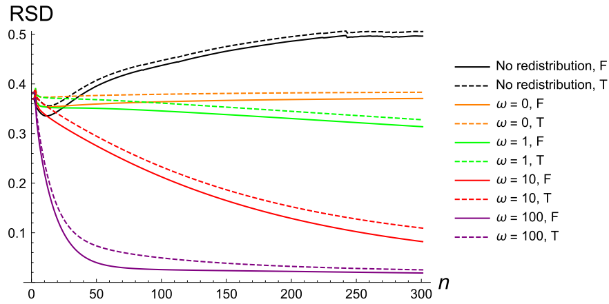
FIGURE 26. The evolution of relative standard deviation (RSD) of the covolume areas for the evolution of cylmng-like shape. The solid lines correspond to \text{RSD}^{F,n} and dashed lines correspond to \text{RSD}^{T,n} .
