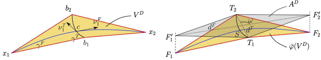
FIGURE 14. The geometry of a diamond cell. Left panel: a diamond cell on the manifold X . Right panel: \bar{\varphi} -image of a diamond cell on \tilde{X}^n .
