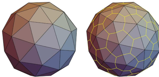
FIGURE 8. A discretization of the sphere S^2 embedded in \mathbb{R}^3 . Left panel: the triangulation \bar{X}^n . Right panel: the triangulation \bar{X}^n and the boundaries \bar{\varphi}^n(\partial V_i) of the finite volumes V_i, i = 1, \dots, n_F .
