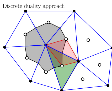
FIGURE 3. Discrete duality method, unknowns both in vertices and cell centers of the primal mesh (Color online).
