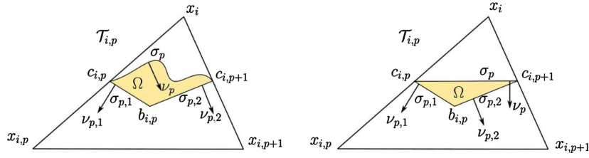
FIGURE 9. Path independence of the integral from c_{i,p} to c_{i,p+1} .
