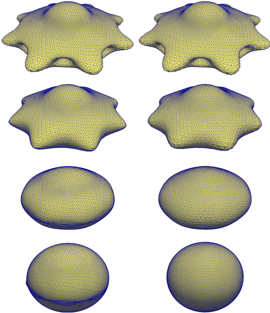
FIGURE 24. The volume preserving mean curvature flow of a cympling-like shape with n_V = 7682 , n_F = 2562 and n_T = 5120 . Both F - and T -finite volume meshes are displayed. Left column : the case with no tangential redistribution. Right column : the evolution with asymptotically uniform tangential redistribution with \omega = 100 . The selected time steps are n = 0, 10, 50, 300 .
