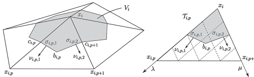
FIGURE 7. Left panel: the finite volume V_i around the vertex x_i . Right panel: the local coordinates on a triangle \mathcal{T}_{i,p} .
