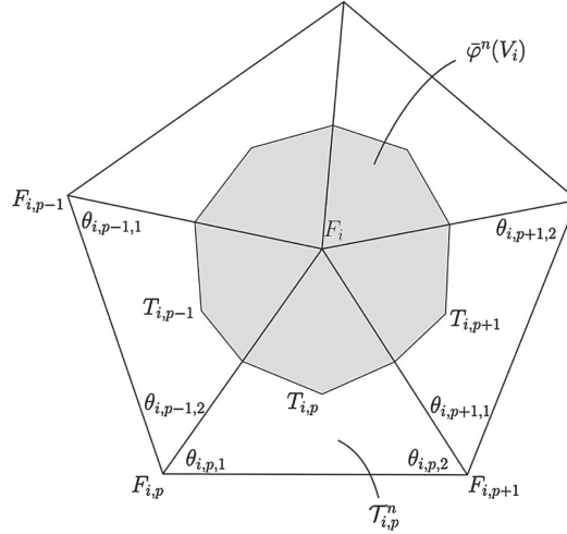
FIGURE 10. Notation around the vertex F_i .
