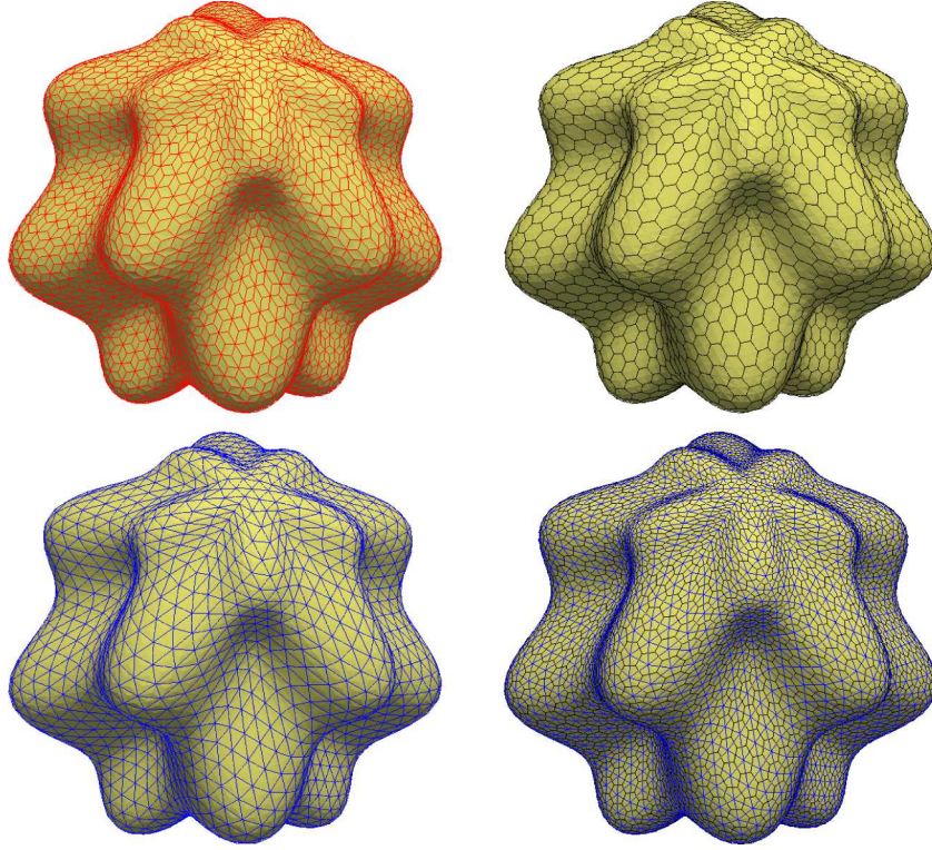
FIGURE 22. A discretization of the bumpy sphere with n_V = 7682 , n_F = 2562 and n_T = 5120 . Edges of various meshes are displayed. From the top left, diamond mesh, F -covolumes mesh, T -covolumes mesh, both F - and T -covolumes meshes.
