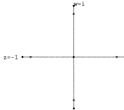
Fig. 2. The normalized dessin of g .
