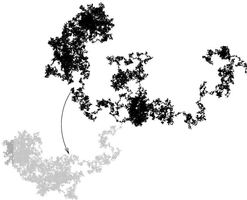
Fig. 1. A pivoting point of angle \pi/2 (in gray is the image of one half of the path by a rotation of angle +\pi/2 ).
