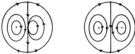
FIG. 8. — There is symmetry, hence graphs are finite
