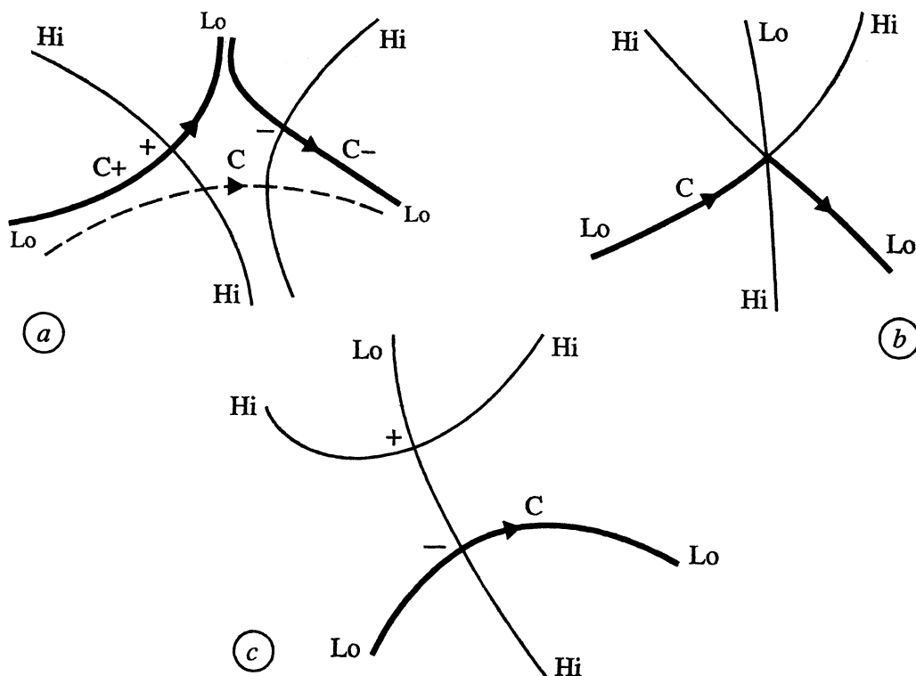
FIG. 1. — Coalescence and separation of saddles in s plane as X varies across the catastrophe set. \text{Hi} and \text{Lo} denote asymptotic ridges and valleys of \text{Re } \Phi ; light lines are steepest paths, i.e. contours of \text{Im } \Phi ; heavy lines are steepest descent contours through the saddles + and - ; the dashed line in (a) is a possible defining contour for the integral. The catastrophe occurs at (b). At (a), both saddles contribute; at (c), one contributes.
