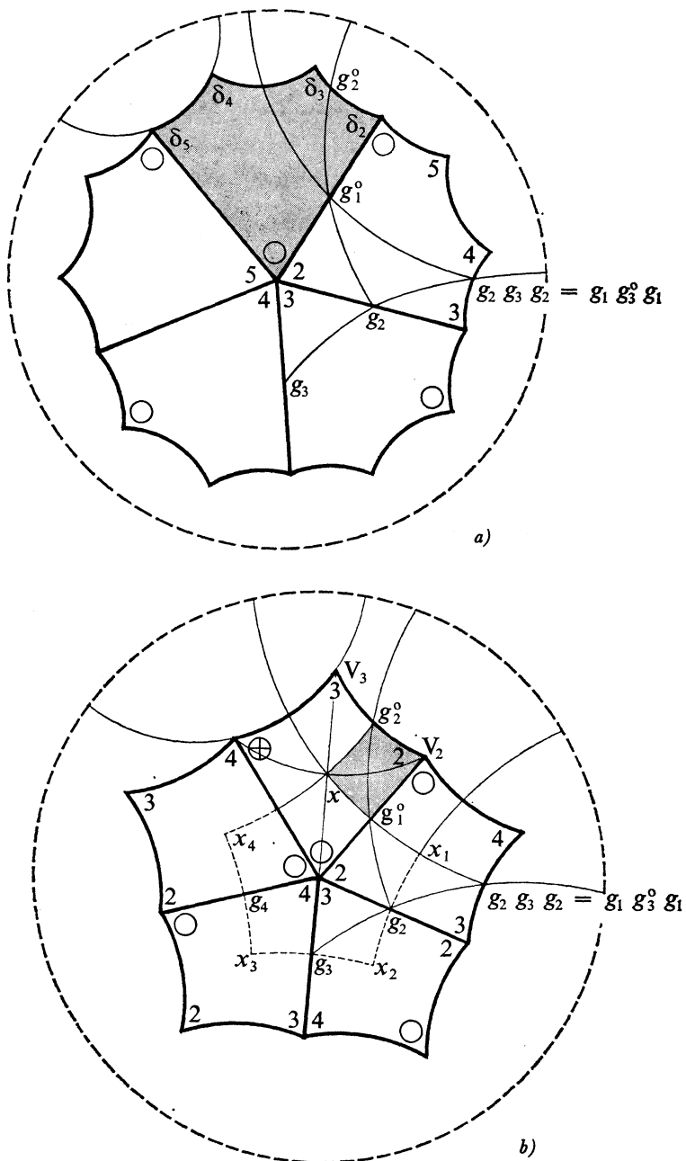
FIG. 2. — a ) (v, n) = (5, 5) ; b ) (v, n) = (4, 5) , x_i = g_i \dots g_2 g_1 x rigid
