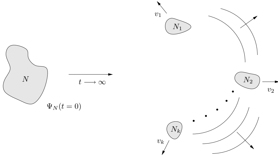
Figure 2: An N -particle state, \Psi_N(t) , evolving, as t \rightarrow \infty , into k \geq 1 bound coherent clusters of bosons with \frac{N_i}{N}\nu > \nu_* , i = 1, \dots, k , receding from each other with velocities, v_i , plus some dispersive “radiation”.
