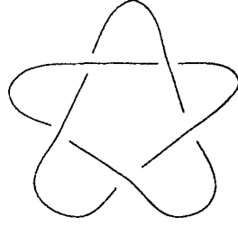
Figure 4: Link diagram for M_{5,0}
