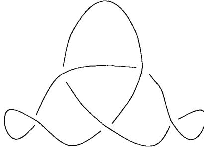
Figure 1: Knot for Poincaré homology sphere
