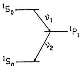
Fig. 6. Radiative cascade emitting pairs of photons correlated in polarization. that only even isotopes can be used 10 ).
