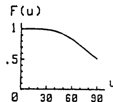
Fig. 9. F(u) for a 0 - 1 - 0 cascade.
