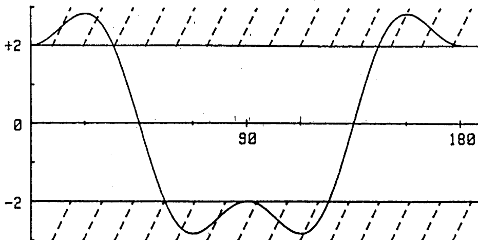
Fig. 5. S(\theta) as predicted by Quantum Mechanics for pairs in state (1). The conflict arises in the '///' zone.
