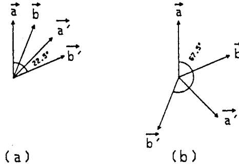
Fig. 4. Orientations yielding the largest conflict between Bell's Inequalities and Quantum Mechanics.
