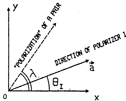
Fig. 2. Our exemple. Each pair has a "direction of polarization," defined by \lambda .
