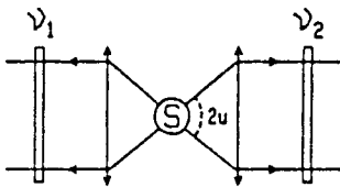
Fig. 8. Realistic configuration, with finite solid angles.
