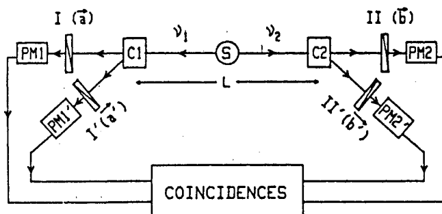
Fig. 14. Timing-experiment with optical switches. ( C_1 and C_2 ). A switching occurs each 10 ns. The two switches are independently driven.
