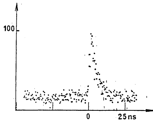
Fig. 11. Time-delay spectrum. Number of detected pairs as a function of the delay between the detections of two photons.
