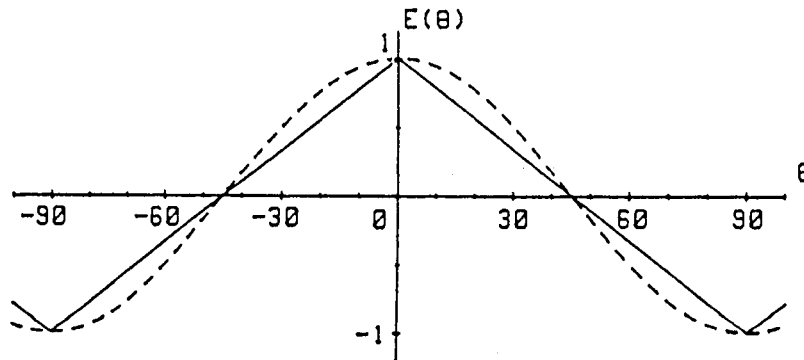
Fig. 3. Polarization correlation coefficient, as a function of the relative orientation of the polarizers.
