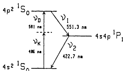
Fig. 10. Two-photon excitation of the chosen cascade in Calcium.
