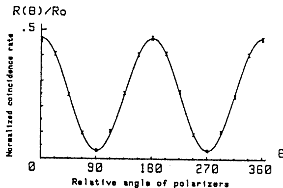
Fig. 12. Experiment with one channel polarizers : Normalized coincidence rate as a function of the relative polarizers orientation. Indicated errors are \pm 1 standard deviation.
