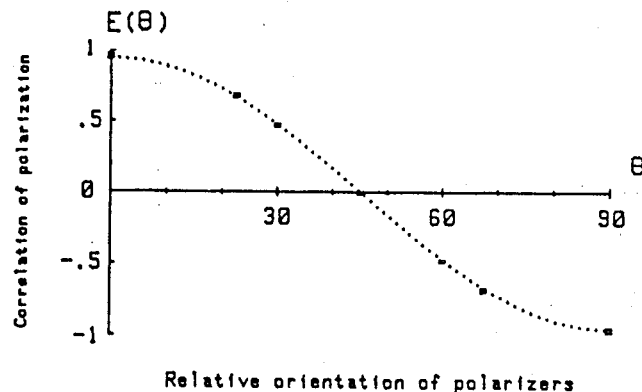
Fig. 13. Experiment with two-channels polarizers : Correlation of polarizations as a function of the relative angle of the polarimeters. The indicated errors are \pm 2 standard deviations. The dashed curve is not a fit to the data, but Quantum Mechanical predictions for the actual experiment. For ideal polarizers, the curve would reach the values \pm 1 .
