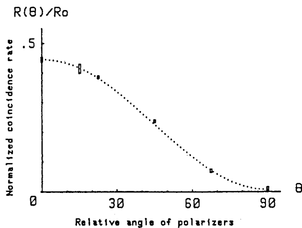
Fig. 15. Timing experiment : average normalized coincidence rate as a function of the relative orientation of the polarizers. Indicated errors are \pm 1 standard deviation. The dashed curve is not a fit to the data but the predictions by Quantum Mechanics for the actual experiment.
