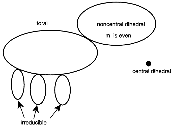
FIG. 2. — The space of conjugacy classes of SO(3, \mathbf{R}) representations of the group G_n^s
