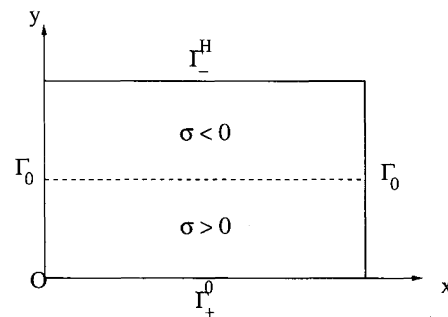
FIGURE 3. \sigma(x, y) = 1 - 2y .
