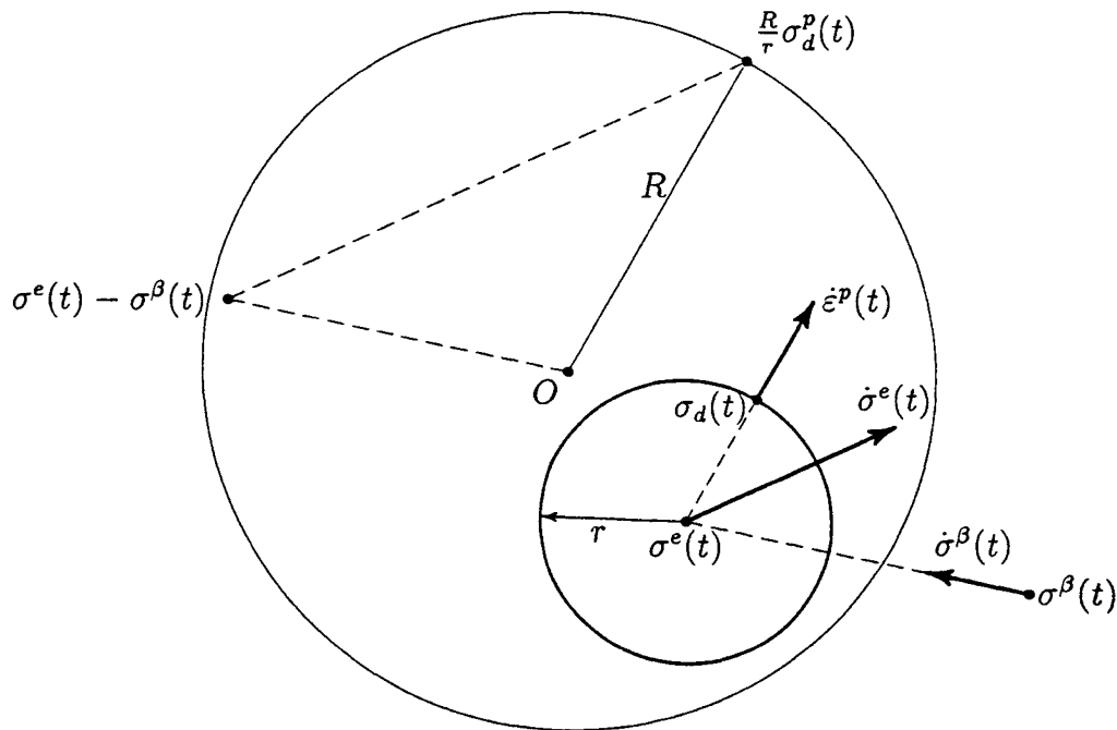
Figure 4. — The model of Bower.
