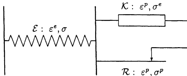
Figure 1. — The rheological model for kinematic hardening.
