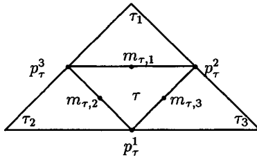
Figure 4.1. — Location of \tau , \tau_i , p_{\tau}^i and m_{\tau,i} , 1 \leq i \leq 3 .
