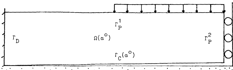
Figure 5.3. — \Omega(\alpha^0) and partition of \partial\Omega(\alpha^0) .
