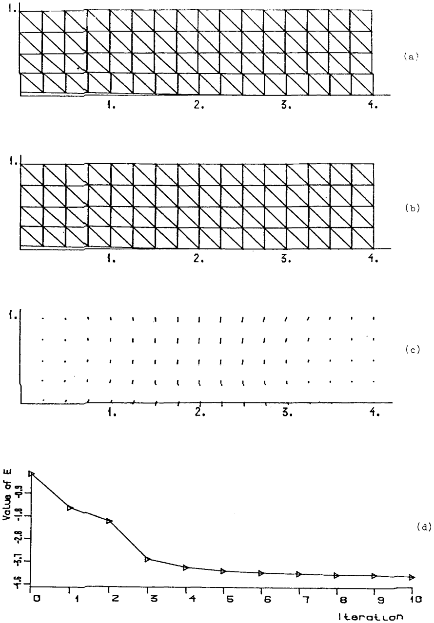
Figure 5.2. — Numerical results for Example 5.1.
