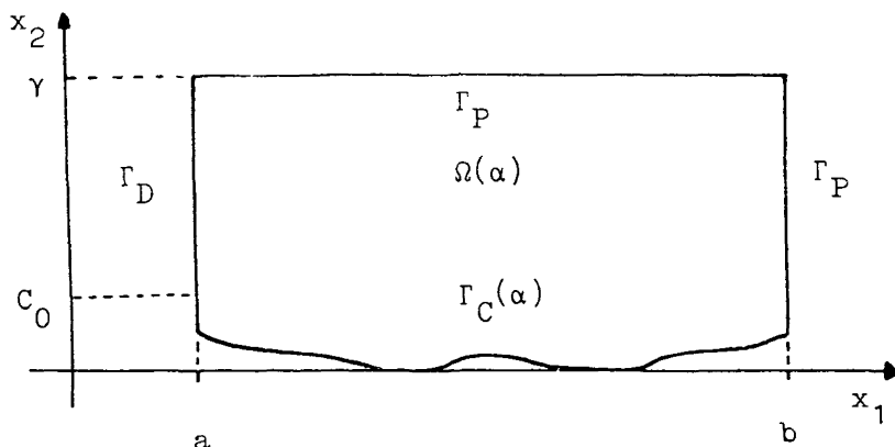
Fig. 2.1 \Omega(\alpha)
