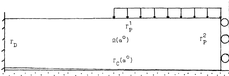
Figure 5.1. — \Omega(\alpha^0) and partition of \partial\Omega(\alpha^0) .
