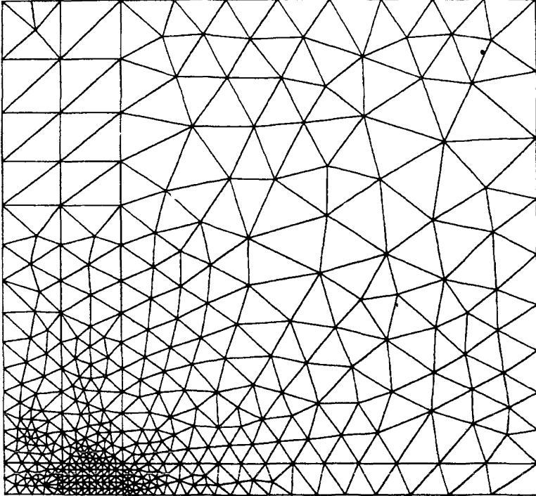
Figure 2. — Detail of the triangulation in figure 1 : The upper subdomain \Omega^+ = (0., 50.) \times (0., 50.) . Number of triangles in \Omega^+ : 725. Number of nodal points : 399. The solution of problem (10.1) was obtained by introducing an homogeneous Neumann's condition on \Gamma_0 = (0., 50) \times \{0.\} .
