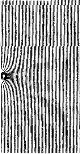
Figure 19. — Streamlines \psi = u - Wr - k = \text{constant} and vorticity region A_\psi = \{ x \in \Omega; x = (r, z), \psi(x) > 0 \} corresponding to the computed solution of (10.1) where \Omega = R(100.) , f is given by (10.18) with \beta = 0.01 , \eta = 20 , and W = 0.7 is prescribed. The computed value of k is 1.348 4.
