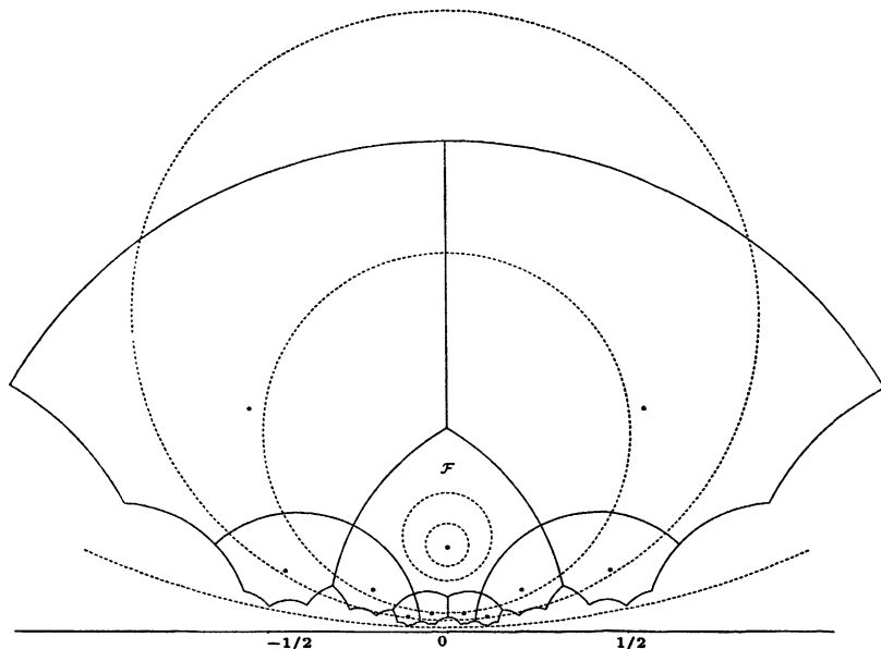
FIGURE 7. Fundamental domains for \Gamma_0^6(1) , and hyperbolic neighborhoods.
