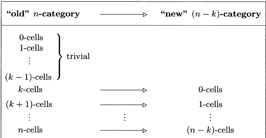
Figure 1: Dimension-shift for k -fold degenerate n -categories
