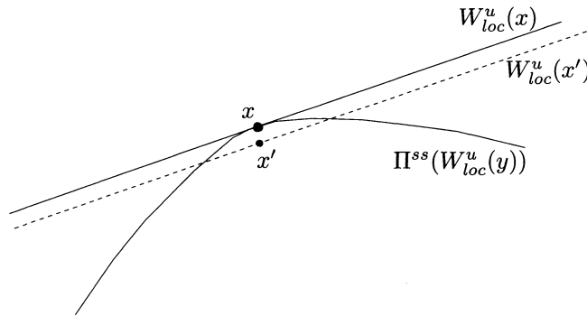
FIGURE 19. Intersection strictement non transverse.
