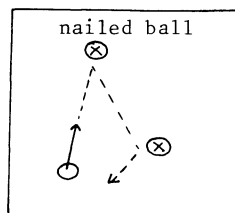
Sinai billiard
