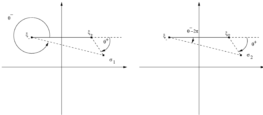
Fig. 1. The two branches of the solution of (2.7), given by (2.8).
