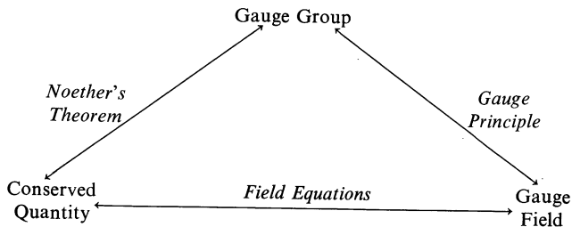
FIG. 1. — The Gauge Triangle.
