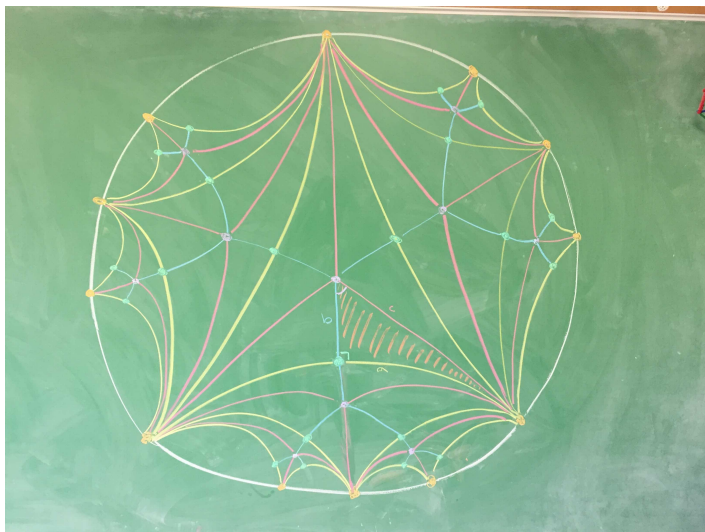
Figure 2.1: A tiling of the hyperbolic plane generated by the reflections in the sides of a triangle with angles \frac{\pi}{2} , \frac{\pi}{3} and 0. The original triangle has been shaded.
