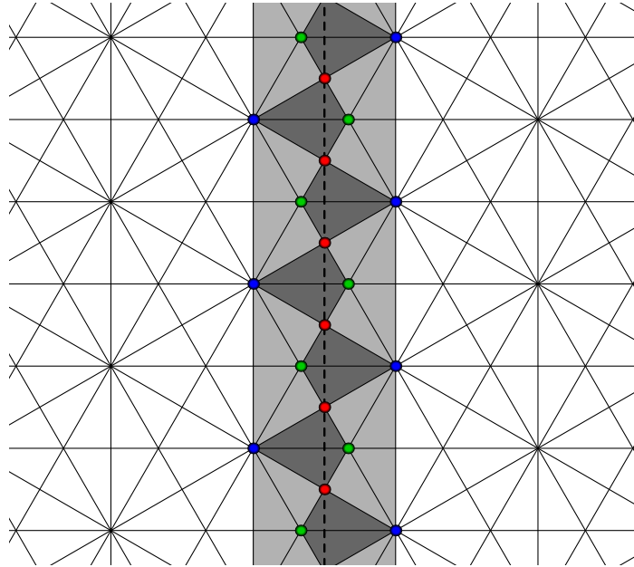
Figure 1.4: The euclidean Coxeter Group \text{Cox}(\tilde{G}_2) .
