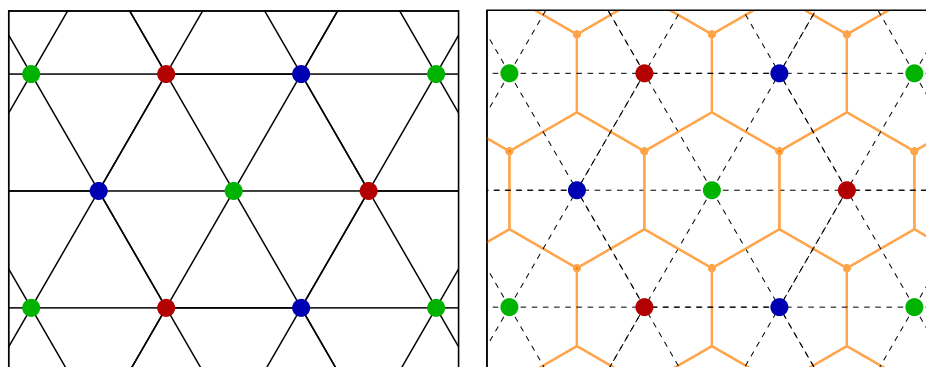
Figure 10.3: A 1-dimensional example of a complex euclidean reflection group and the corresponding Voronoi cell decomposition.
