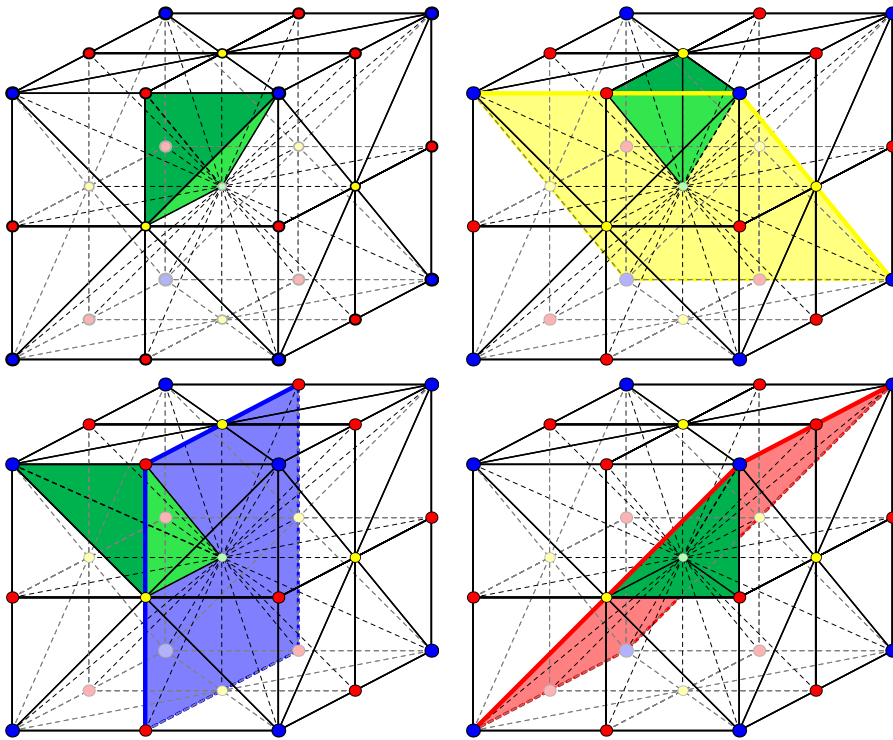
Figure 1.1: The spherical Coxeter group Cox(B_3) .
