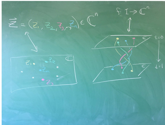
Figure 4.1: The Braid Arrangement
