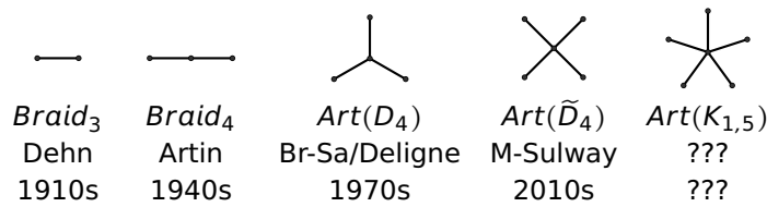
Figure 8.1: The slow progress in understanding the word problem for Artin groups defined by stars.
