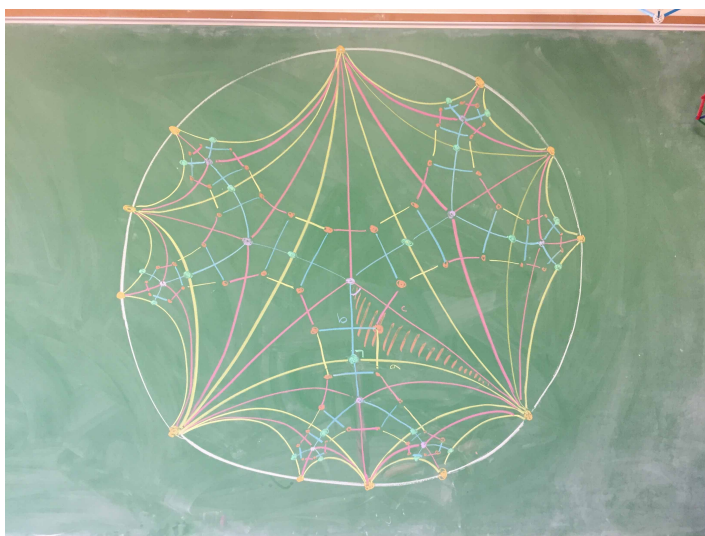
Figure 3.1: A portion of the Cayley graph of our running example superimposed on the corresponding triangular tiling of the hyperbolic plane.
