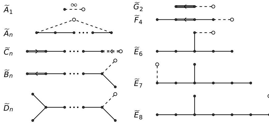
Figure 1.3: Four infinite families and five sporadic examples.
