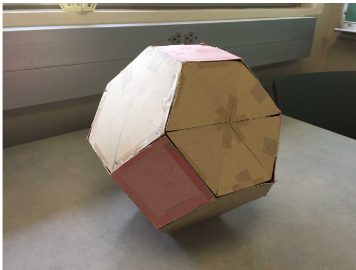
Figure 1.2: The Sym_4 Permutahedron.
