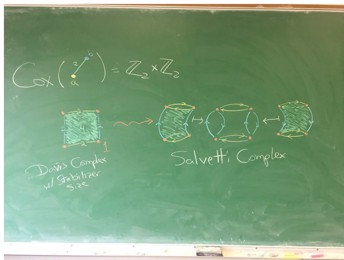
Figure 4.2: An example of the Salvetti complex as an oriented version of the Davis complex.
