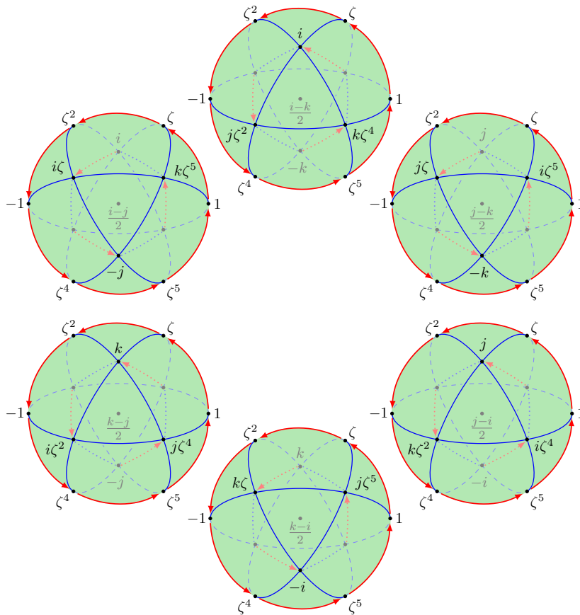
Figure 10.2: Six lenses that together display the structure of the 24-cell. Each figure represents a one-sixth lens in the 3-sphere with dihedral angle \frac{\pi}{3} between its front and back hemispheres. They are arranged so that every front hemisphere is identified with the back hemisphere of the next one when ordered in a counter-clockwise way.
