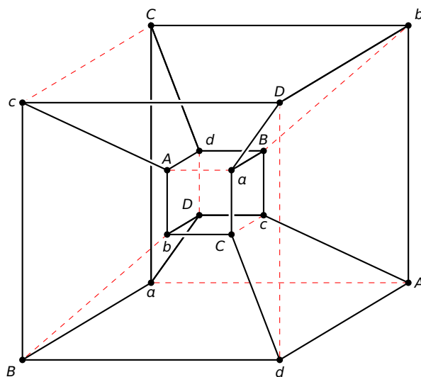
Figure 10.4: The Möbius-Kantor graph.
