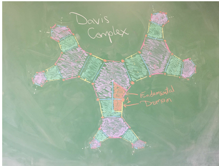
Figure 3.2: A portion of the Davis complex for our running example.
