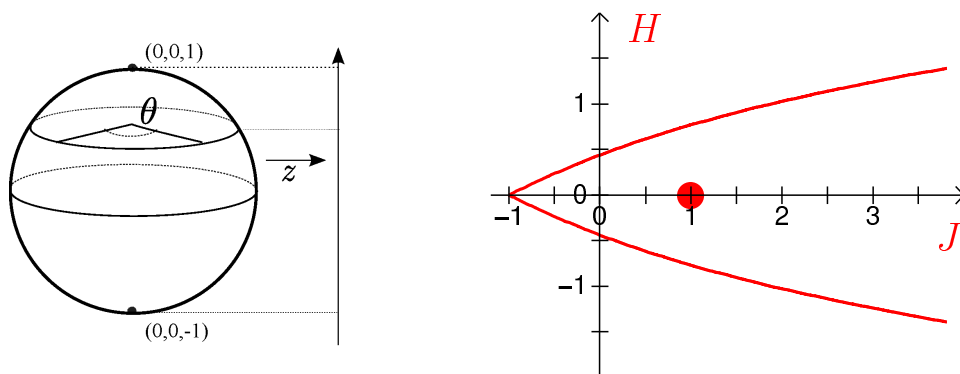
Figure 4: The figure on the right shows the bifurcation diagram of the classical spin-oscillator system.
