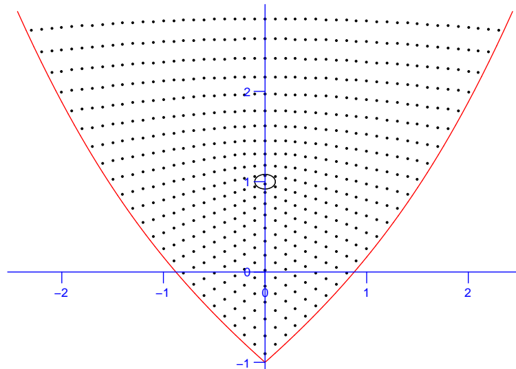
Figure 3: Joint spectrum of the Spherical pendulum. The peculiar arrangement of eigenvalues around the point (0, 1) is a characterization of quantum monodromy.
