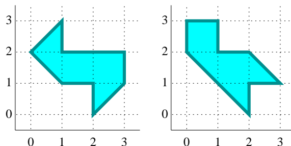
Figure 1: An example of non-isometric polygonal domains with the same spectrum, found by Gordon, Webb, Wolpert.
