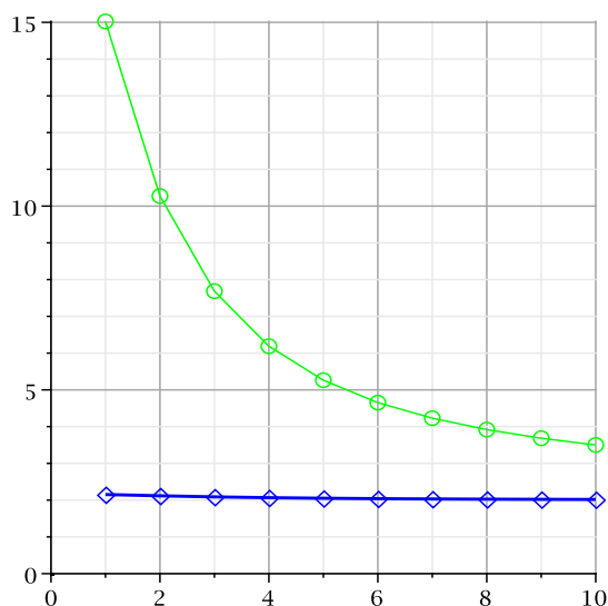
Figure 6: Recovering dynamical invariant B . The abscissa is logarithmic : it is an integer k such that \hbar = 1/(2^{k-1} + 1) . Thus the classical limit \hbar \rightarrow 0 is observed for large k . The top curve is the naive computation, the bottom one is an accelerated formula taking into account an assumed asymptotic expansion. They show a good convergence to B = 2 .
