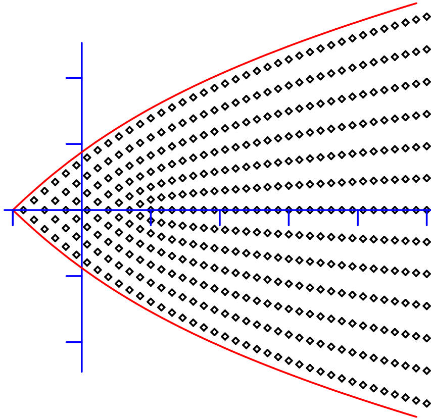
Figure 5: The joint spectrum of the spin-oscillator.
