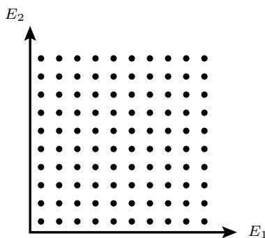
Figure 2: Joint spectrum of harmonic oscillators. It extends indefinitely in the positive quadrant.
