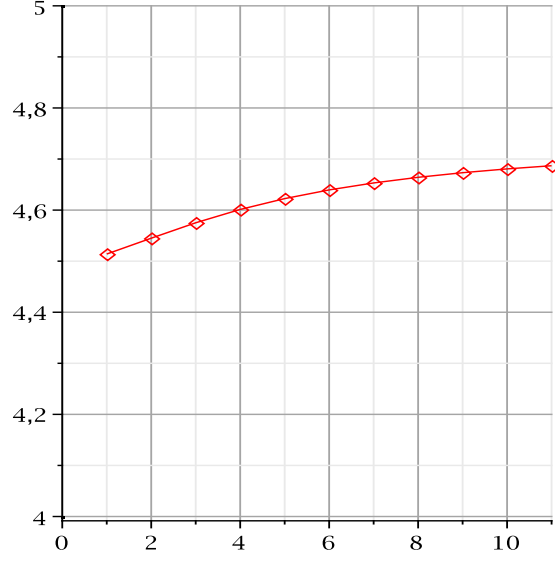
Figure 7: Recovering dynamical invariant a . The abscissa is the same as in Figure 6. We find from this plot a \simeq 4,7 .
