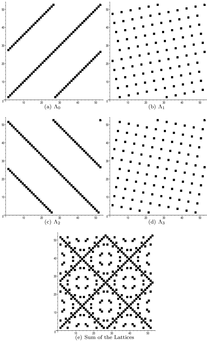
FIGURE 4. Combining the lattices
