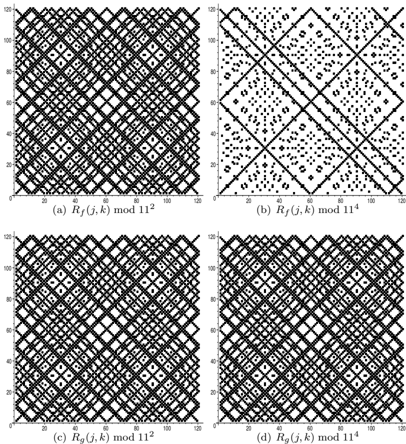
FIGURE 3. Periodicity modulo 11^2 and 11^4
