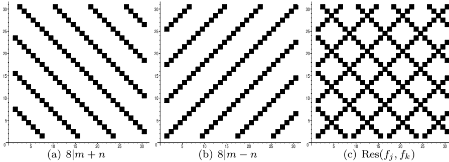
FIGURE 5. f = x^2 - 3x + 1
