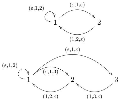
FIGURE 1. The prefix-suffix automata corresponding to the Fibonacci (above) and the Tribonacci substitution (below).
