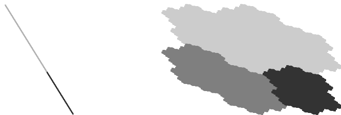
FIGURE 2. The atomic surfaces associated to the Fibonacci (left) and the Tribonacci (right) substitution.
