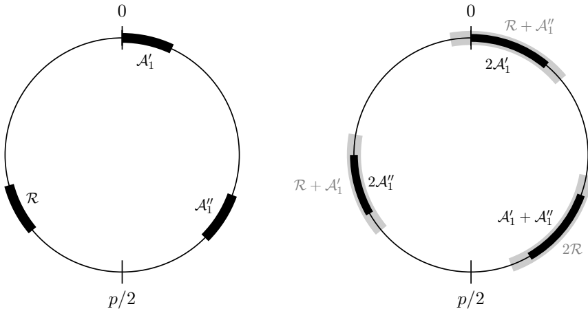
FIGURE 3.1. Distribution of \mathcal{A} and 2\mathcal{A} in \mathbb{Z}_p in case (iii).
