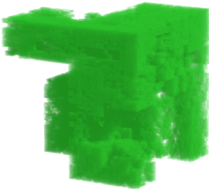
FIGURE 4.7. A 3-dimensional random Kakeya set over \mathbb{Q}_2
