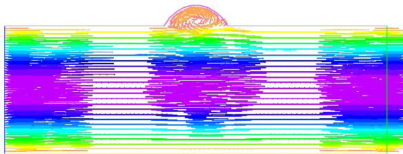
(b) Optimal shape for J_1 and J_3 , min. and max. speed: 0. and 5.00.
