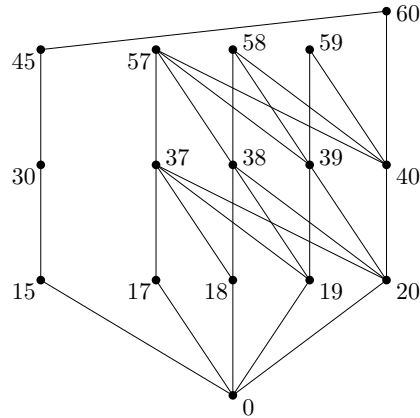
FIGURE 5. \text{Ap}(\mathcal{S}, 16) for \mathcal{S} = \langle 15, 16, 17, 18, 19, 20 \rangle .
