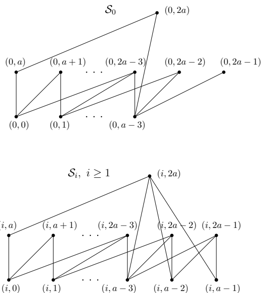
FIGURE 8. \mathcal{S}_0 and \mathcal{S}_i for i \geq 1 .
