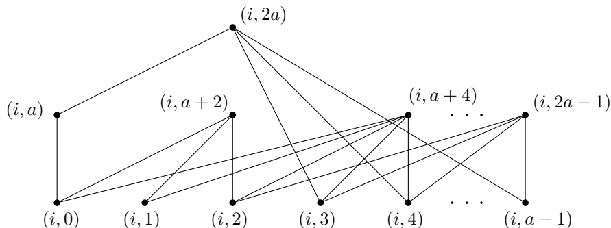
FIGURE 12. P \cap \mathcal{S}_i in case (5).
