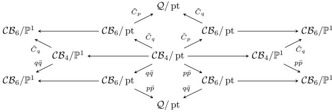
Figure 2.5. A disc of type 4.
