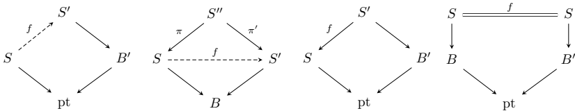
Figure 2.1. From left to right: Sarkisov link f of type I, II, III and IV.
