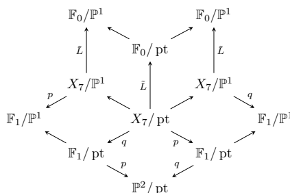
Figure 2.6. A disc of type 5.
