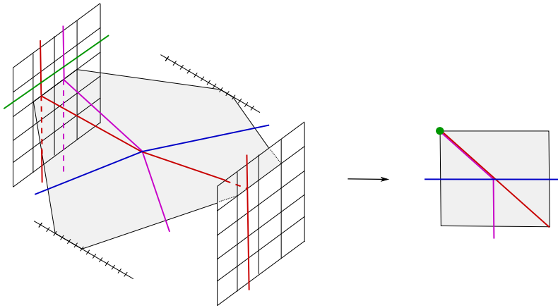
Figure 3.4. Examples of the three types of walls of \mathcal{E}G (left) and their associated hypergraphs in X (right), in the case A = \mathbb{Z}^2, B = \mathbb{Z} . To avoid a busy picture, we only represent the case of a polygon of X with 4 sides. Blue: Walls/Hypergraphs associated with edges of X . Green: Walls/Hypergraphs associated with edges of \mathcal{E}G_{bal} of first type. Red and pink: Walls/Hypergraphs associated with edges of \mathcal{E}G_{bal} of second type.
