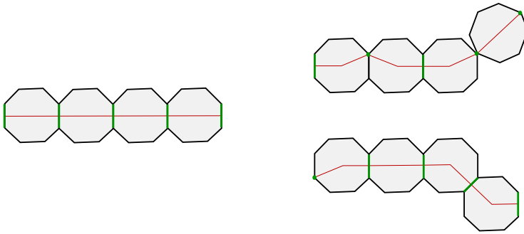
Figure 3.1. Examples of hypercarriers with their associated hypergraphs (in red) and doors (in green). Configurations on the left are studied in detail in [33]. The configurations on the right are studied in detail in the appendix.
