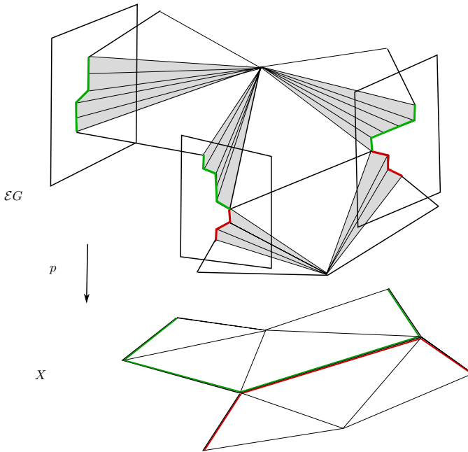
Figure 2.3. The polyhedrons of \mathcal{E}G . The figure presents portions of two simplicial polygons of X (one green, one red) and its preimage in \mathcal{E}G . Vertical triangles are shaded. Attaching paths in the various fibres are coloured with respect to the associated polygon of X .
