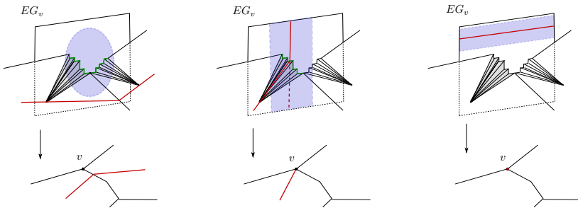
Figure 4.1. The three possible configurations, depending on the relative position of the hypergraph associated with W_i and the vertex v . In red: walls and hypergraphs. In green: K_i . In blue: C_i .
