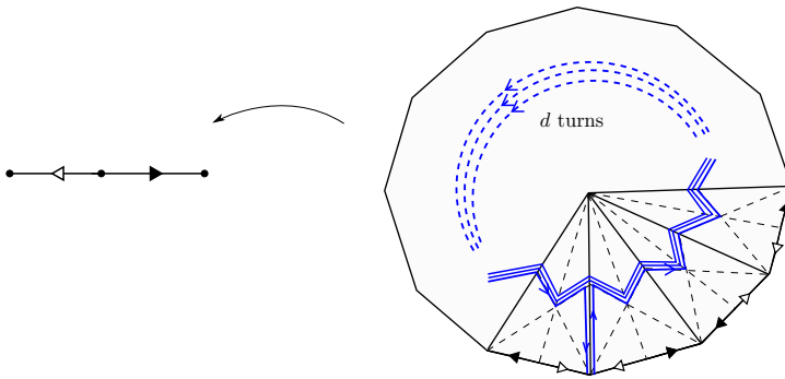
Figure 2.2. A homotopically trivial G(\mathcal{K}'_{\text{simpl}}) -loop.
