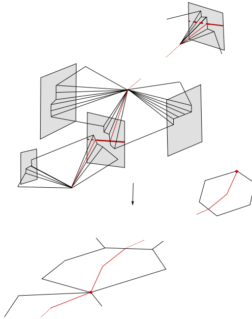
Figure 3.2. A portion of a wall associated with an edge of \mathcal{E}G_{bal} of second type, together with its hypergraph. To avoid drawing too many edges, we assume here that \mathcal{E}G is balanced, that is, \mathcal{E}G = \mathcal{E}G_{bal} .
