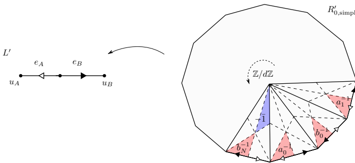
Figure 2.1. Part of the complex of groups G(\mathcal{K}'_{simpl}) . Twisting elements corresponding to white triangles of R'_{0,simpl} are trivial. (The element \bar{1} denotes the generator of \mathbb{Z}/d\mathbb{Z} .)
