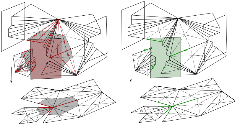
Figure 3.3. The construction of the projection map q_v . The star of v and its preimage in \mathcal{E}G_{bal} are represented in shaded. On the left, the various radial projections \tilde{R} \cap S(v) \rightarrow \partial\tilde{R} \cap S(v) . On the right, the various projections \partial\tilde{R} \cap S(v) \rightarrow EG_v .
