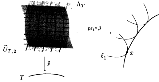
Figure 4.2. Proof of Theorem 1.4
