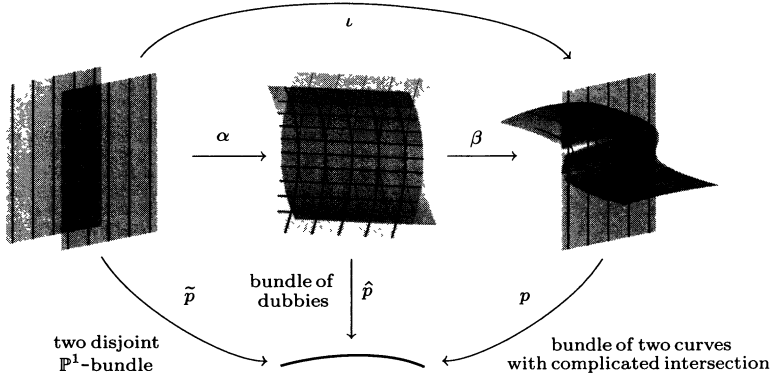
Figure 3.1. A partial resolution of singularities
