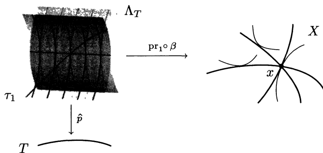
Figure 4.1. Proof of Theorem 1.4
