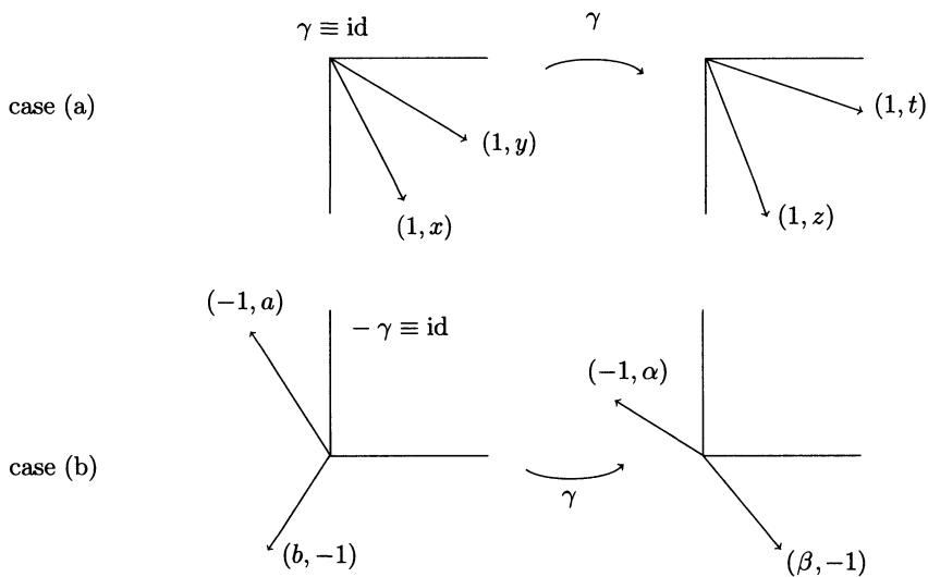
Figure 3. Notation for Corollary 10 — application of the Morita formula — cases (a) and (b)
