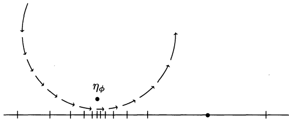
Figure 5. The backward trajectory of a point corresponding to a saddle-node cascade
