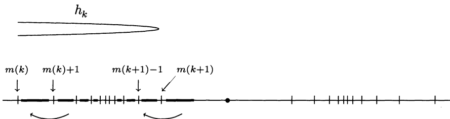
Figure 2. A long saddle-node cascade
