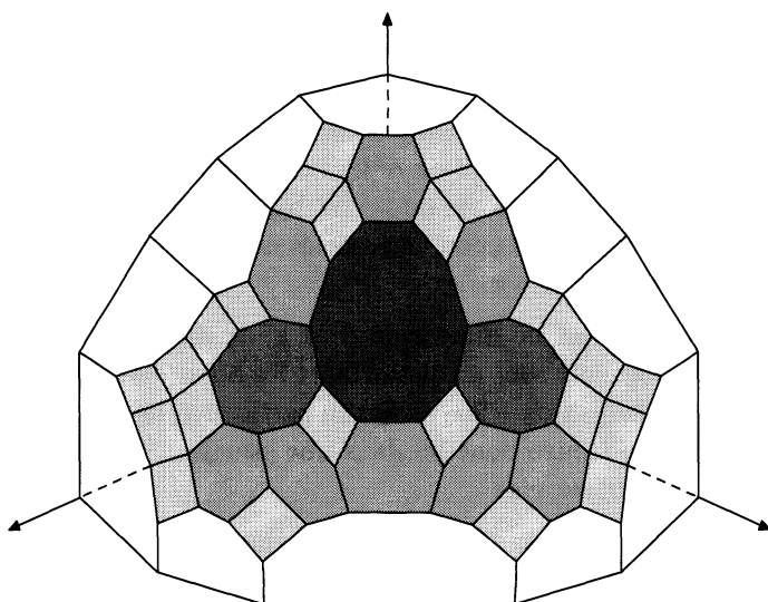
Figure 15. Le polyèdre \mathcal{C}_{\mu,3,4} .
