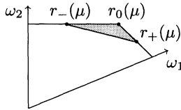
Figure 10. Le polygone C_{\mu,2,3} .
