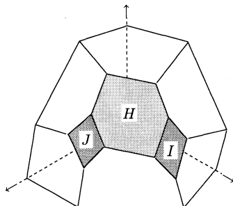
Figure 14. Le polyèdre \mathcal{C}_{\mu,2,4} .
